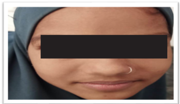
Figure2 Granulomatous Inflammation
